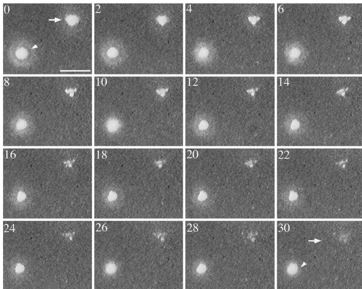
FIGURE 3 DNA packaging-like event of a class 2 DNA molecule. T7 DNA was added to a p6-supplemented T7 3,5,6 DNA-metabolizing extract. Fluorescence microscopy was performed after incubation for 60 min. In a search for internal transformations of concatemers, videotaped images were reviewed. An active class 2 DNA molecule is indicated by an arrow in the first and last frames (time (s) is indicated at the upper left). As described in the text, changes in this molecule are observed in intermediate frames. An inactive class 2 DNA molecule is indicated by an arrowhead in the first and last frames. The length of the bar is 10 \mu m.
