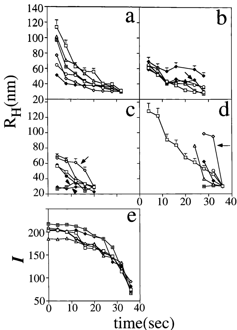
FIGURE 4 Quantitative analysis of DNA packaging-like events observed by light microscopy. The following are plotted as a function of time for DNA packaging-like events. (a–c) R_H for each lobe of three class 2 DNA molecules in a T7 3.5 DNA-metabolizing extract; (d) R_H for the class 2 DNA molecule imaged in Fig. 5 (low temperature preparation); (e) I for each lobe of a class 2 DNA molecule in a T7 3.5 extract. One-half the experimental error in R_H at any given time is indicated for all plots by a vertical bar in the uppermost plot of a–d. The time span of the plots varies for the following reasons: the time of the first data was limited, in all cases, by separation of lobes sufficient for tracking. In the case of a–c and e, the time of the first data was also limited by the time at which videotaping began. The class 2 DNA molecule used for (a) is also used for (e).
