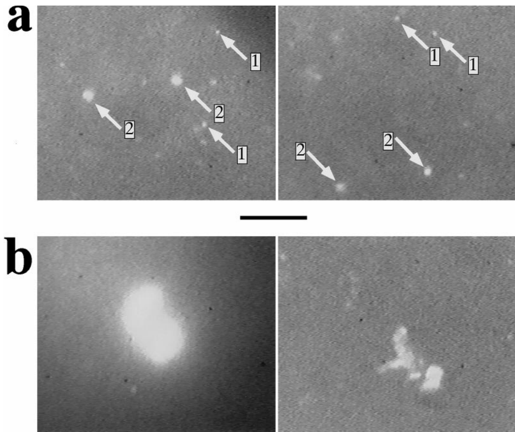
FIGURE 2 DNAs cleaved from a DNA network. After adding T7 DNA to a T7 3,5 DNA-metabolizing extract, incubation was performed at 30°C. The DNA-extract mixture was observed by fluorescence microscopy at 60 min after the start of incubation. (a) Fields that contain particles most of which appear to be single DNA molecules. (b) Fields that contain aggregate-like particles. The length of the bar is 10 \mu m.
